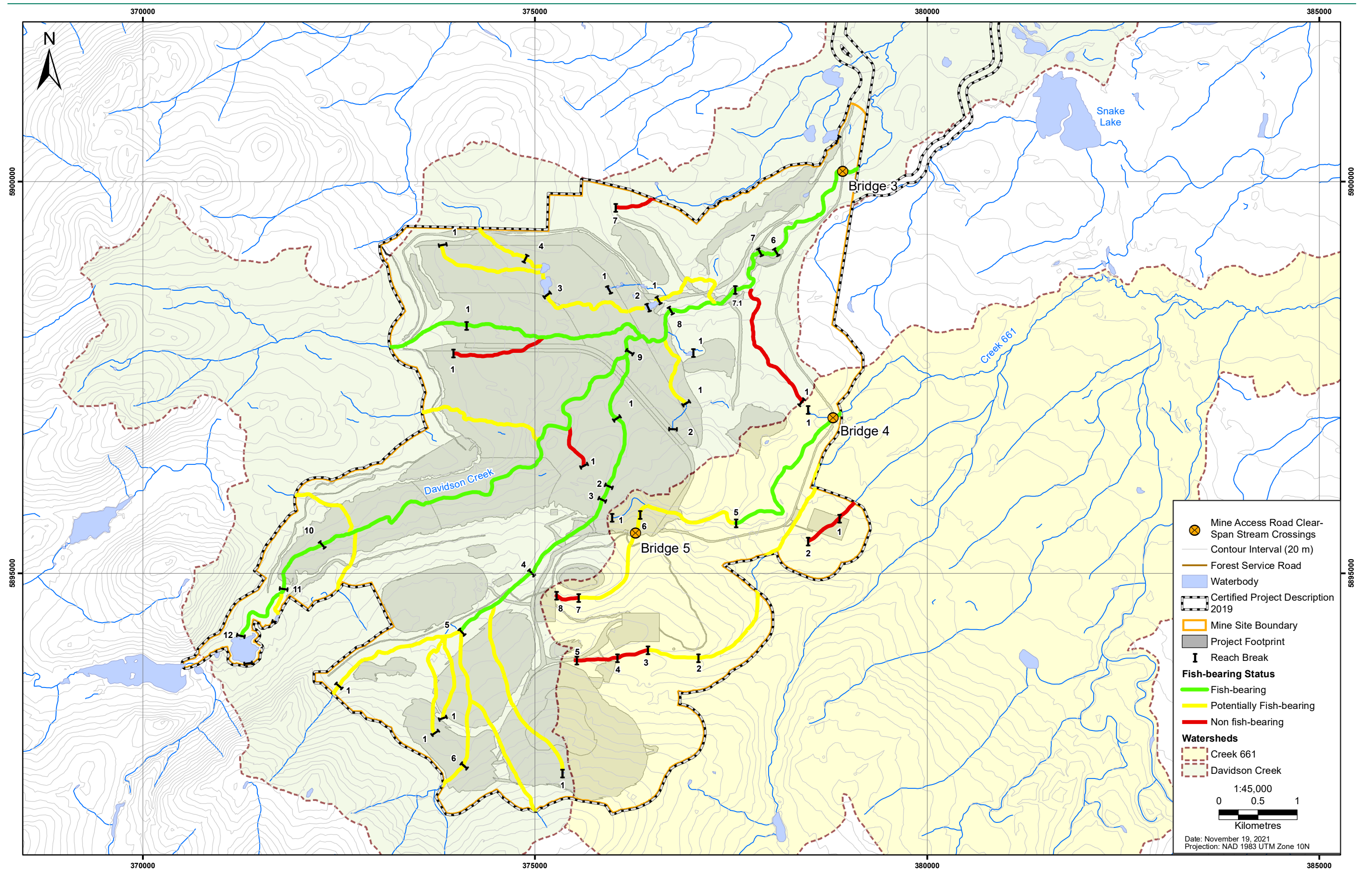
Figure 3.5-1: Fish Bearing Streams and Fish Habitat Quality within the Mine Site
